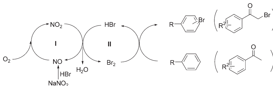
Scheme 3. Plausible catalytic mechanism for the oxybromination by oxygen.
